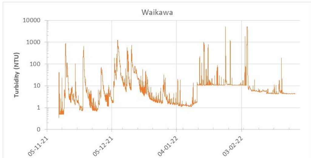
Figure H.4: Turbidity logger in Manakau Stream and the Waikawa Stream (30-minute median of 10-minute readings).
